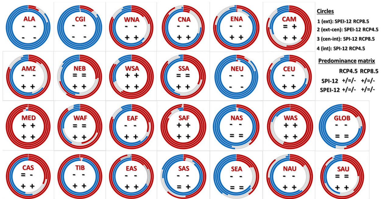
FIG. 9. Percentage of areas projected to experience an increase (red) or decrease (blue) in both drought frequency and severity from 1981–2010 to 2071–2100. Gray refers to either mixed or not robust changes. The inner circles refer to SPI-12 (internal: RCP4.5; central-internal: RCP8.5), the outer circles to SPEI-12 (central-external: RCP4.5; external: RCP8.5). The “predominance matrix” reports the dominant tendency: + (–) means that more than 50% of the areas show a simultaneous increase (decrease) in both DF and DS, = means that the simultaneous increase and decrease occurs in less than 50% of the areas.
