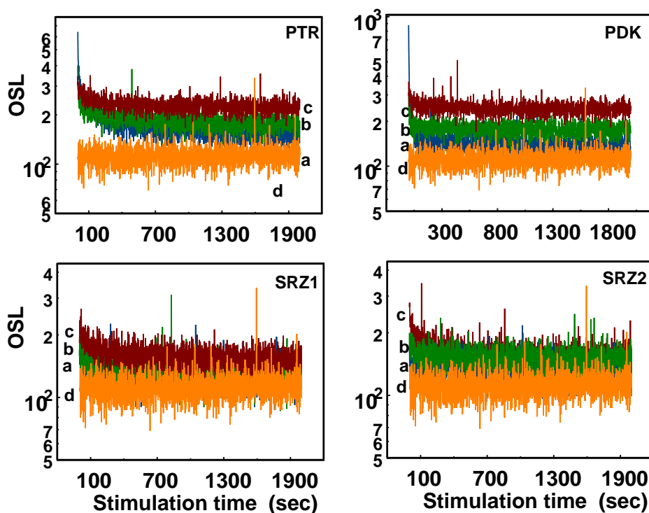
Figure 2: Low efficiency TT-blueOSL curve shapes for quartz measured at various OSL measuring temperatures. Curve (a) 190 °C, Curve (b) 250 °C and Curve (c) at 375 °C. Curve (d) corresponds to the background OSL signal measured at room temperature
