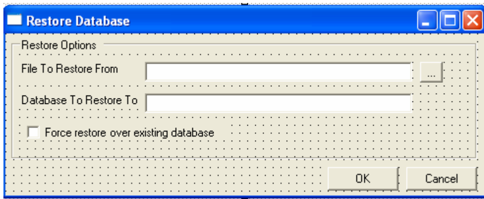
Figure 5.6 Restore Database
