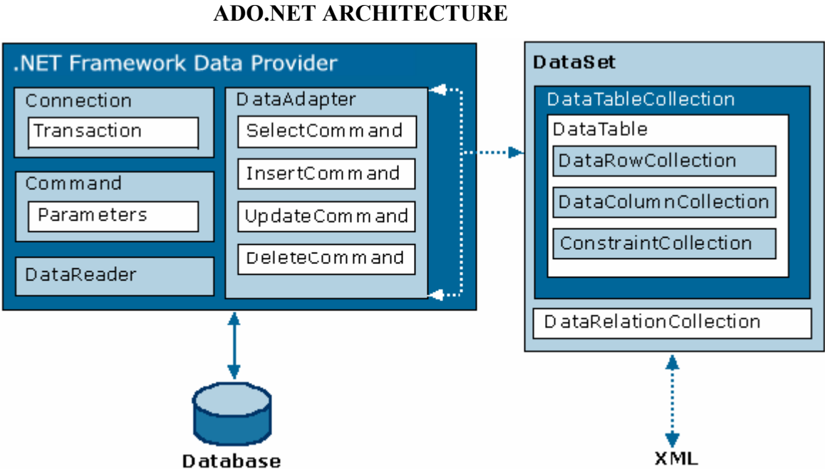
Figure 3.2 ADO.NET Architecture
