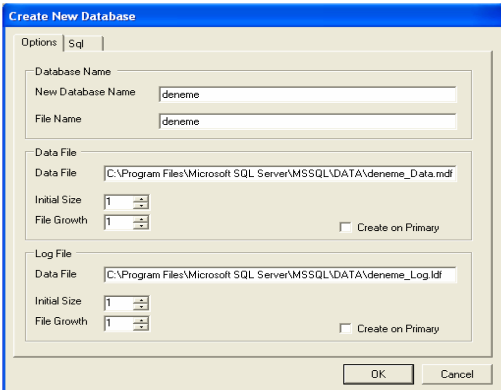
Figure 5.4 New Database
