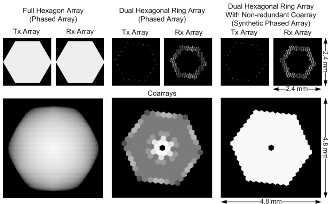
Figure 7.2. Tx-Rx array structures and corresponding coarrays for full hexagon, dual hexagon and dual hexagon with non-redundant coarray.
